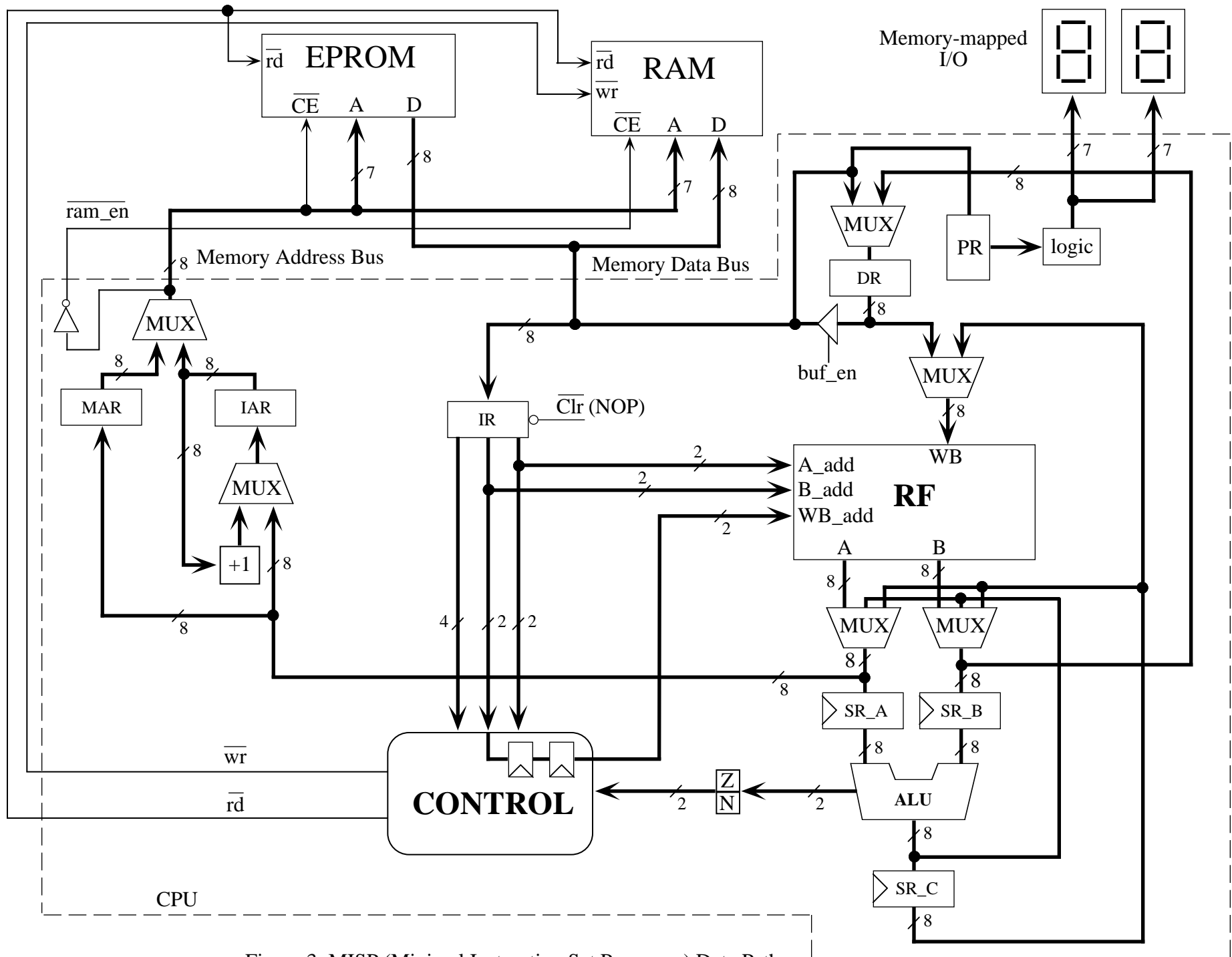
Figure 3: MISP (Minimal Instruction Set Processor) Data Path
