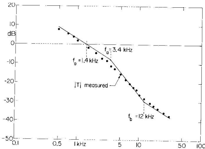
Figure 7. Loop-gain magnitude versus frequency plot obtained by voltage ratio measurements at point A_v in the circuit of Fig. 5.
