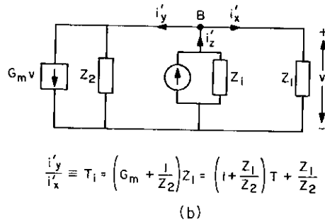
Figure 13. Successive signal injection at the (accessible) point B of arbitrary impedance ratio Z_2/Z_1 in the circuit of Fig. 12, (a) voltage injection and measurement of T_r , (b) current injection and measurement of T_i .
