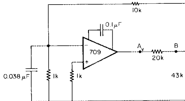
Figure 5. Feedback amplifier circuit for demonstration of loop-gain measurement with voltage injection at point A_r .
