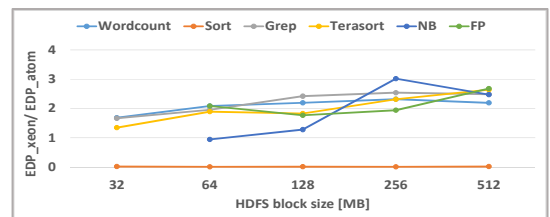
Figure 7: EDP of Hadoop benchmarks at various HDFS block size
