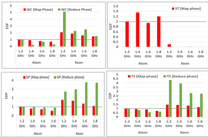
Figure 5: EDP analysis of Map and Reduce phase of (a) WordCount (b) Sort (c) Grep (d) Terasort on big and little core with frequency scaling
