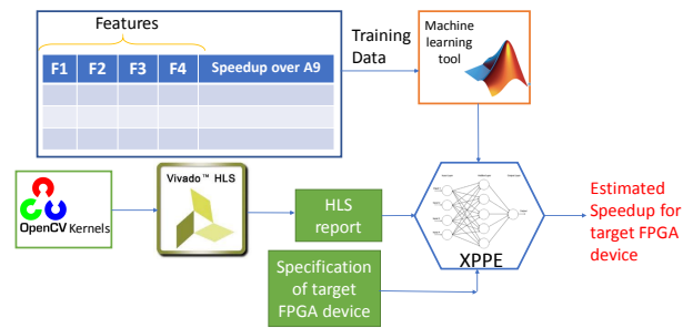
Figure 2: Overall flow of XPPE
