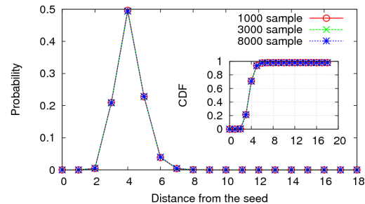
Figure 4: Degree of separation
