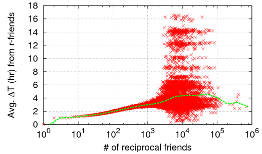
Figure 5: The average time differences between a user and r-friends
