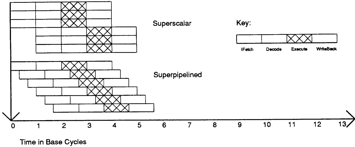
Figure 11: Start-up transient in superscalar vs. superpipelined execution
