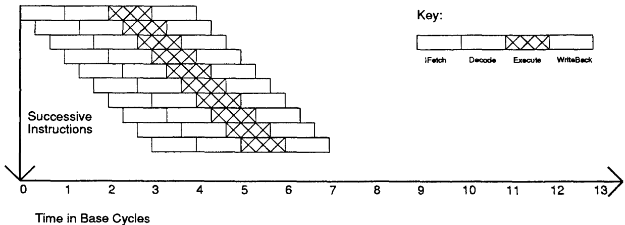
Figure 7: Execution of instructions in a superpipelined machine ( m=3 )
