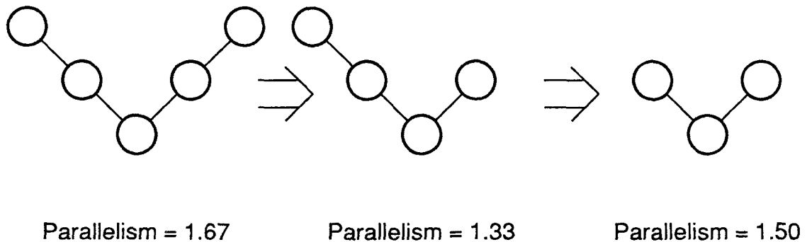
Figure 16: Instruction-level parallelism vs. compiler optimizations
