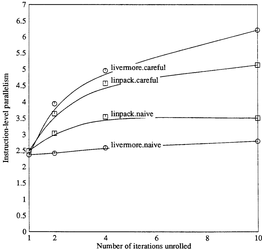
Figure 15: Instruction-level parallelism vs. loop unrolling
