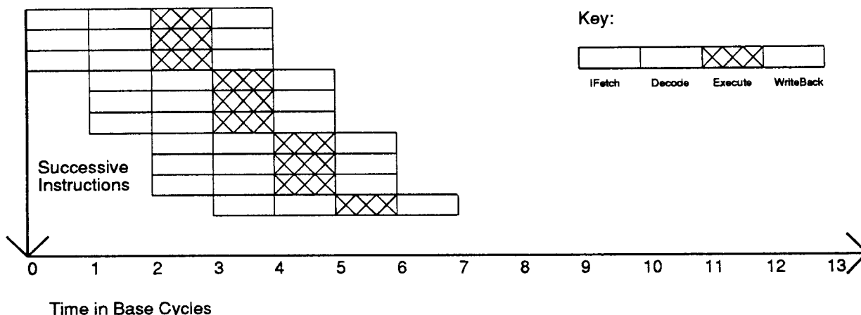
Figure 5: Execution of instructions in a superscalar machine ( n=3 )
