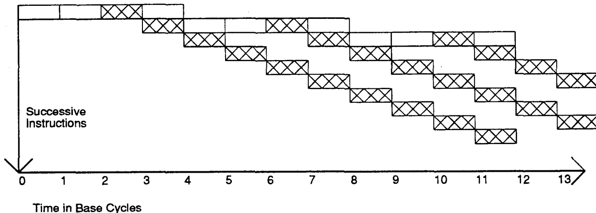
Figure 9: Execution of instructions in a vector machine
