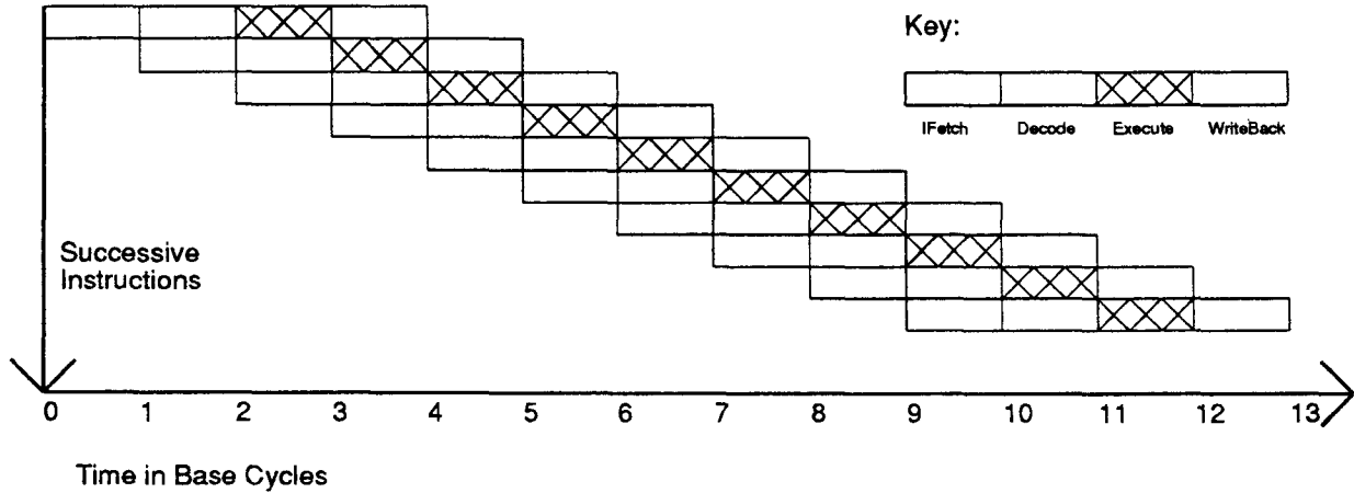
Figure 2: Execution of instructions in a base machine
