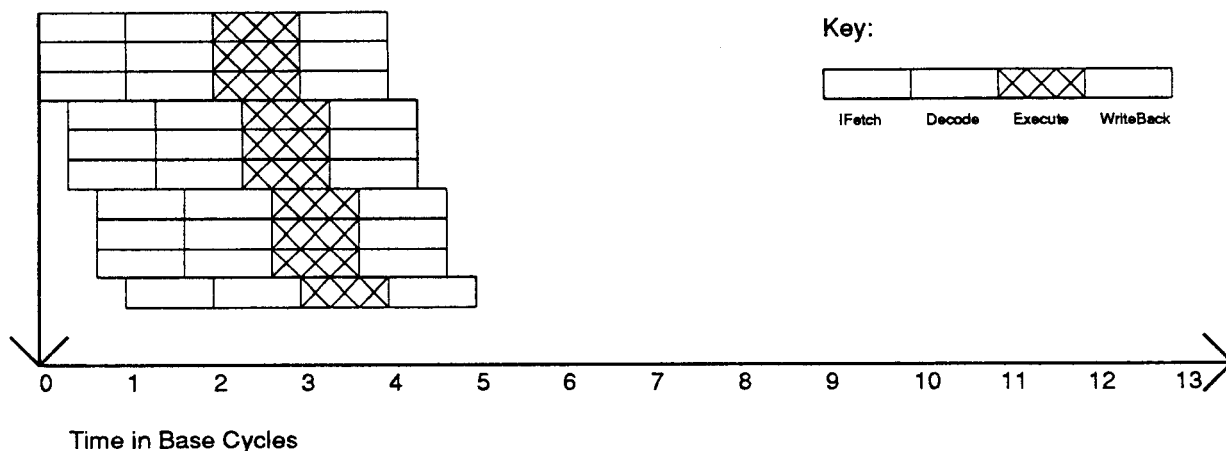
Figure 8: Instruction execution in an superpipelined superscalar machine ( n=3, m=3 )
