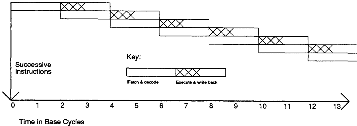
Figure 3: An underpipelined machine with cycle time greater than a simple operation latency
