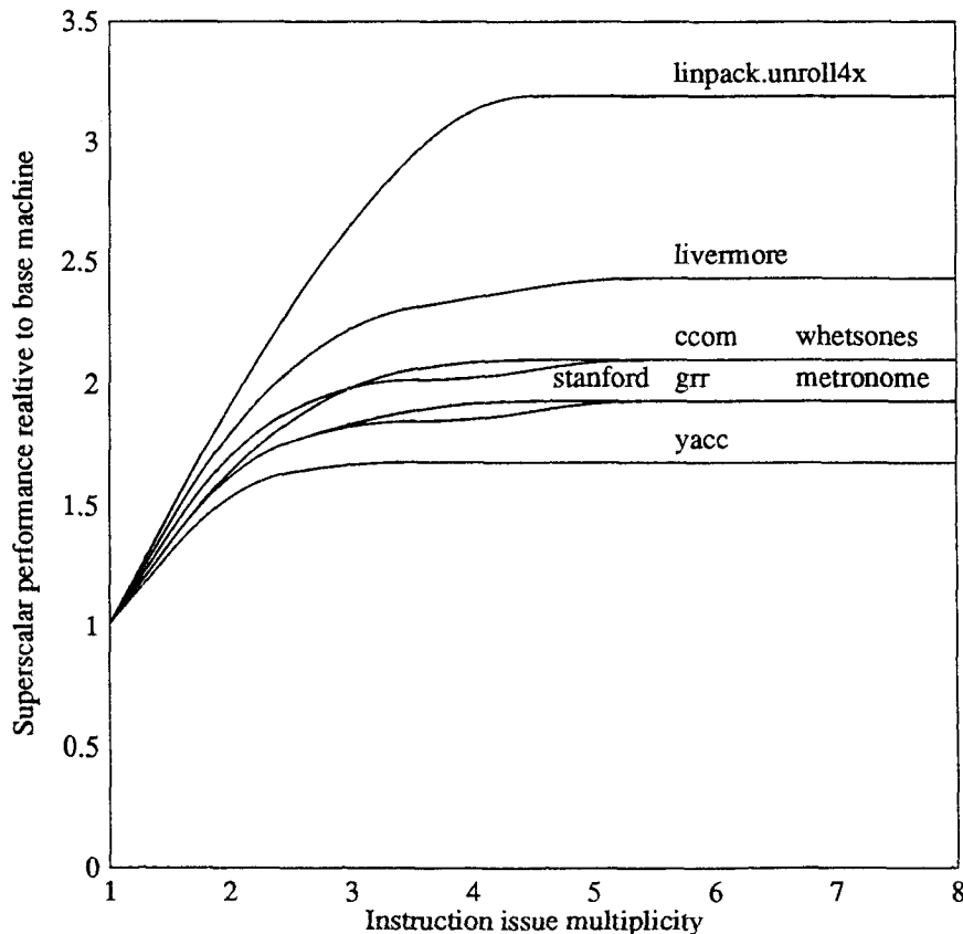
Figure 14: Available instruction-level parallelism by benchmark
