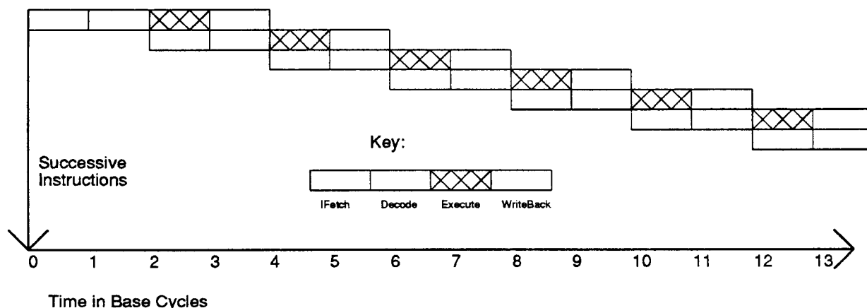
Figure 4: An underpipelined machine that issues less than one instruction per cycle
