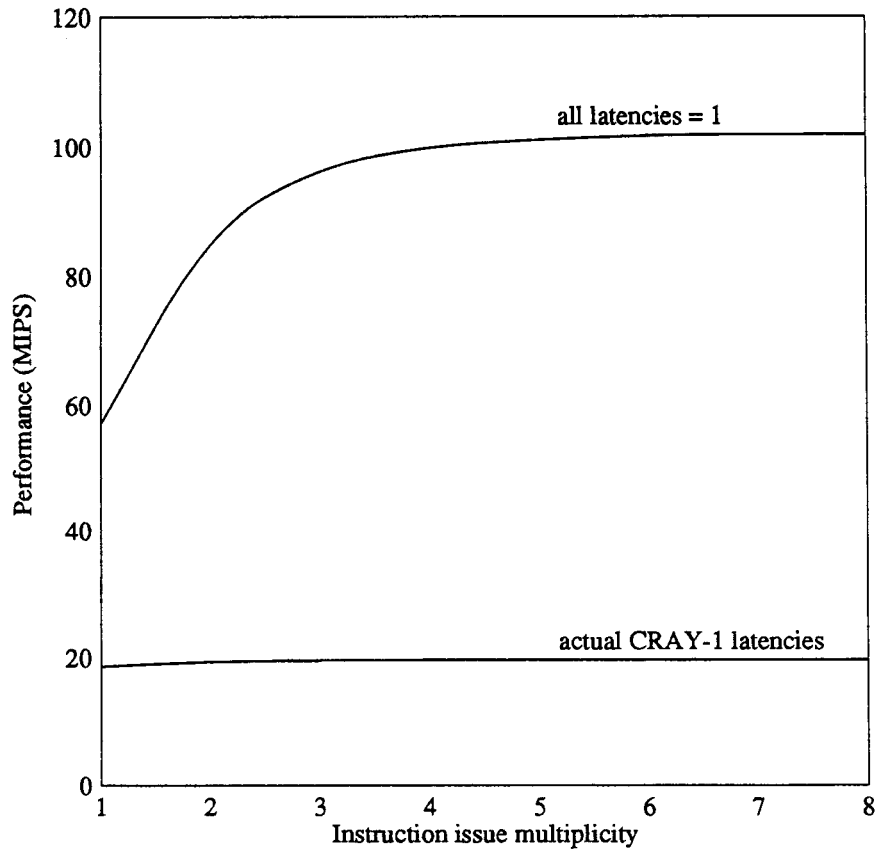
Figure 13: Parallel instruction issue for the CRAY-1 with and without realistic latencies
