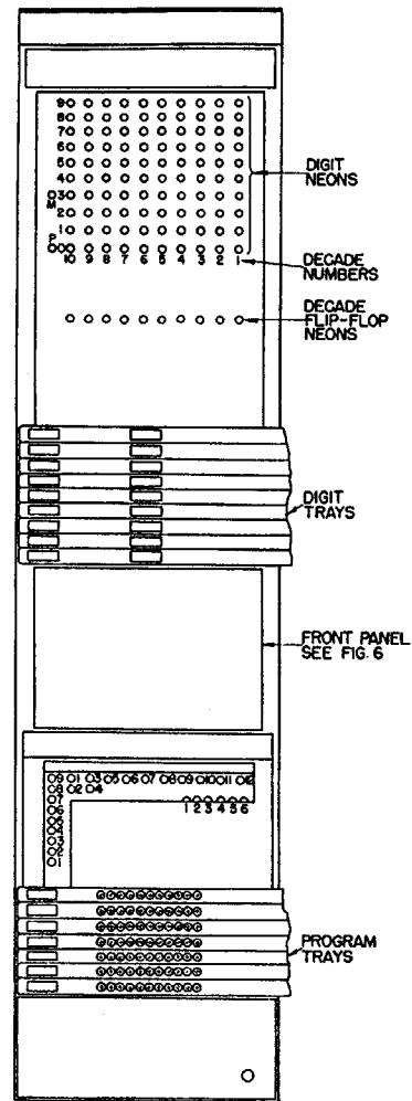
Fig. 5. Front view of an accumulator.
