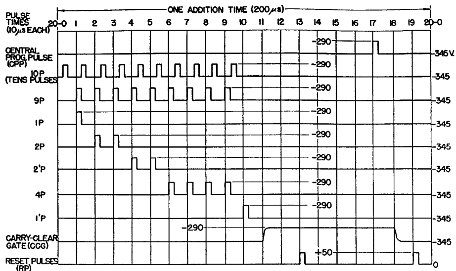
Fig. 1. Pulses used in the operation of the ENIAC.
