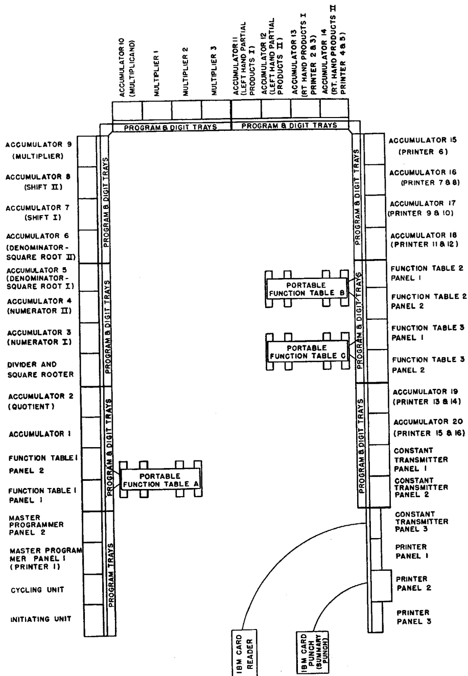
Fig. 2. ENIAC floor layout. Initiating unit—Controls for power, operation controls. Cycling unit—Source of pulses used in operation of ENIAC; name is derived from cycle of pulses shown in Fig. 1 and does not refer to cycles of arithmetic operations. Master programmer—Controls the cycles of arithmetic operations and performs other programming functions. Function table panels—Used in conjunction with function table to call up at high speed numbers “set” in function table. Accumulator—Performs additions and subtractions, stores results, and so forth. Divider—Performs divisions and also can be used to take square roots. Multiplier—Performs multiplications. Constant transmitter—Receives at low speed information from the input device (an International Business Machines card reader, as indicated) or other device, and supplies this information at high speed when called for (note that the input device is at what appears to be the next to the last position rather than at the “beginning” of the ENIAC; this is of no significance). The constant transmitter also has a limited capacity for storing numbers set on switches on its front panel. Printer—Receives at high speed results to be recorded and transmits them to the relatively slow-speed output device (an International Business Machines card punch as indicated). Digit trunks—Special transmission lines into which connection can be made to transmit numbers from one part of the ENIAC to another. Program trunks—Special transmission lines into which connection can be made to transmit program orders (electric pulses) from one part of the ENIAC to another. Trunk from cycling unit—Permanently connected to other units to which it supplies the group of pulses shown in Fig. 1 every 200 microseconds when ENIAC is in continuous operation.
