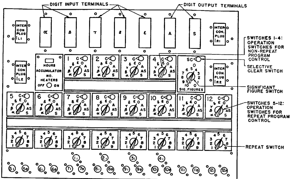
Fig. 6. Accumulator front control panel. Terminals 1i, 2i, \dots, 12i —Program input terminals. Terminals 5\theta, 6\theta, \dots, 12\theta —Program pulse output terminals.
