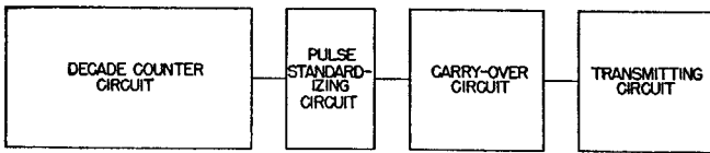
Fig. 4. Block diagram of decade unit.
