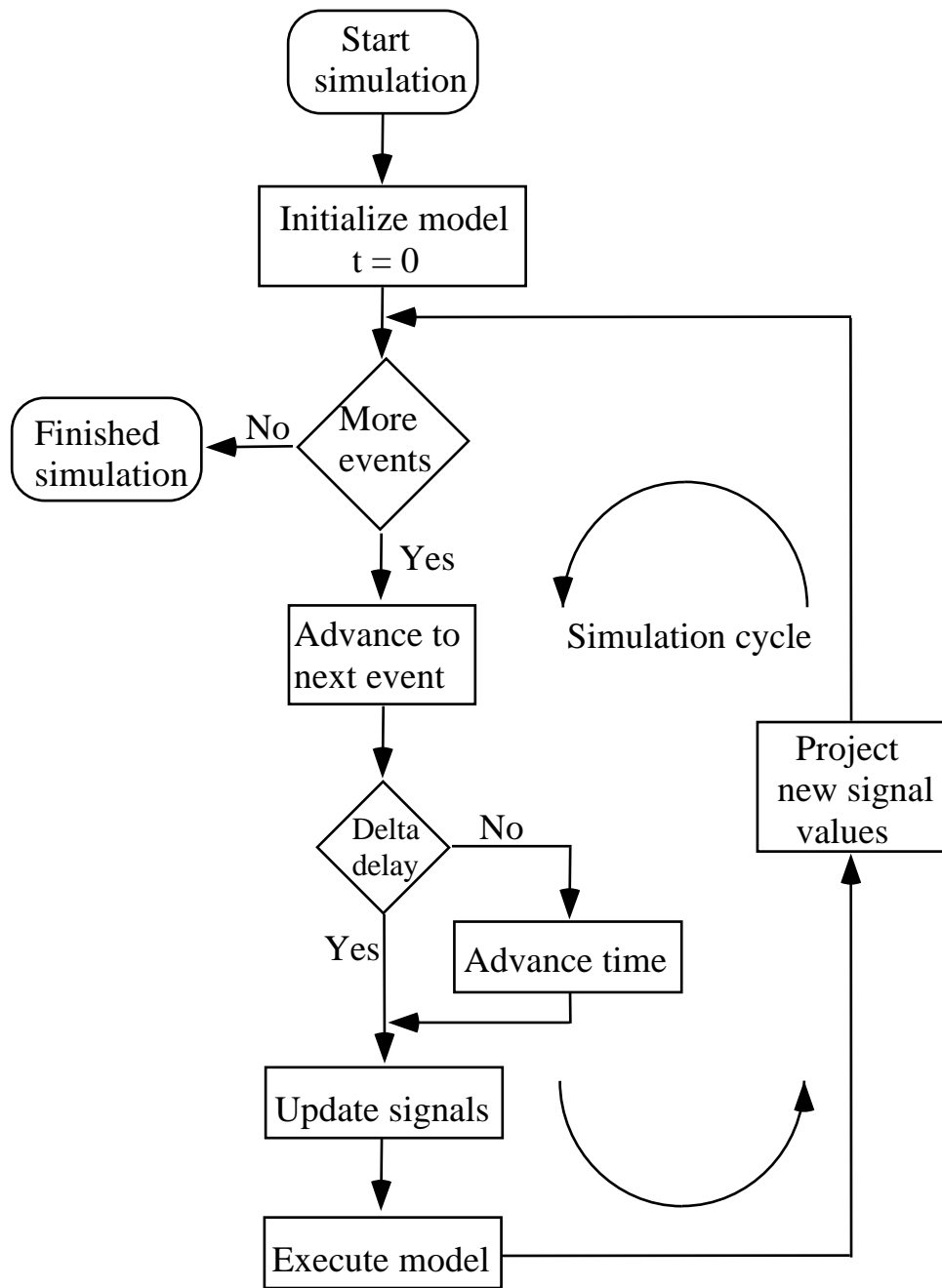
Simplified diagram of VHDL simulation cycle -from Figure 17.18 Allen Dewey, Analysis and Design of Digital Systems with VHDL
