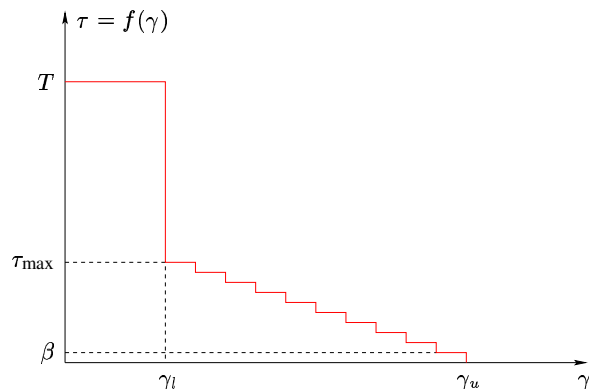
Fig. 4: Backoff function under significant propagation delay
