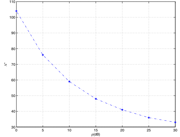
Fig. 6: The optimal number of activated sensors. ( W = 1\text{kHz} , T = 0.01\text{s} , P_{\text{tx}} = 0.181\text{w} , e_c = 1.8\text{nw} ).
