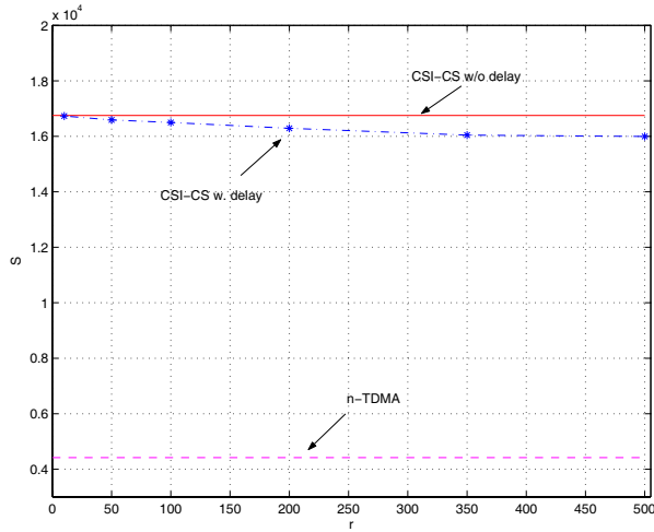
Fig. 5: Performance of CSI-based carrier sensing under significant delay ( \Lambda = 100 , W = 1\text{kHz} , \rho = 3\text{dB} , T = 0.01\text{s} , P_{\text{tx}} = 0.181\text{w} , P_{\text{rx}} = 0.18\text{w} , e_c = 1.8\text{nw} ).
