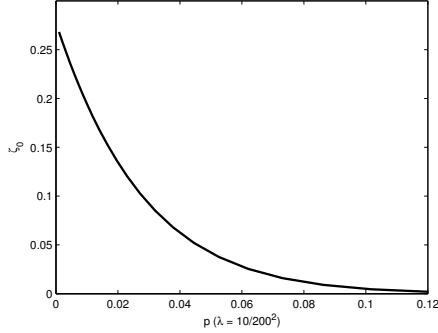
Fig. 5. Critical value of \zeta vs. primary traffic load.
