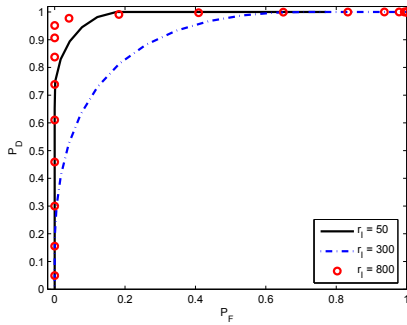
Fig. 4. ROC for LBT ( p = 0.01 , \lambda = 10/200^2 , R_p = 200 , R_I = R_p/0.8 = 250 , d = 0.9 \cdot r_I )
