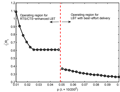
Fig. 7. r_I^* vs p ( \lambda = 10/200^2 )
