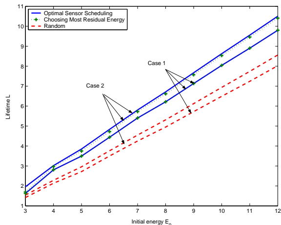
Fig. 1. Lifetime comparison. N = 2 , L = 3 . In case 1, channels are i.i.d.: \Pr\{w_n = 1\} = \Pr\{w_n = 2\} = \frac{1}{4} , \Pr\{w_n = 3\} = \frac{1}{2} for n = 1, 2 . In case 2, channels are non-identically but independently distributed: \Pr\{w_1 = 1\} = \Pr\{w_1 = 2\} = \frac{1}{4} , \Pr\{w_1 = 3\} = \frac{1}{2} , \Pr\{w_2 = 1\} = \Pr\{w_2 = 3\} = \frac{1}{4} , \Pr\{w_2 = 2\} = \frac{1}{2} .
