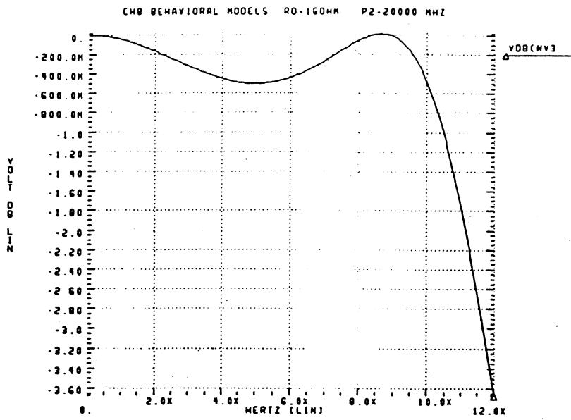
Figure 8.15 Behavioral simulation of the filter of Fig. 8.14, using r_o=1\text{Gohm} , p_2 at 20GHz
