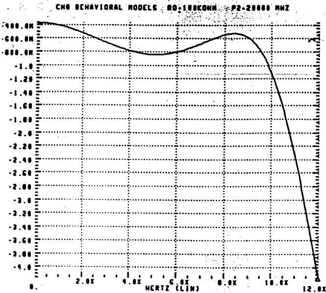
Figure 8.16 Behavioral simulation of the filter using r_o=100\text{Kohm} and p_2 at 20 GHz
