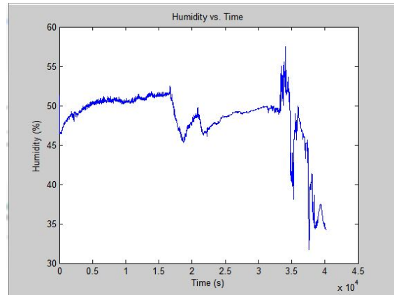
Figure 22: Data captured from live test of humidity
