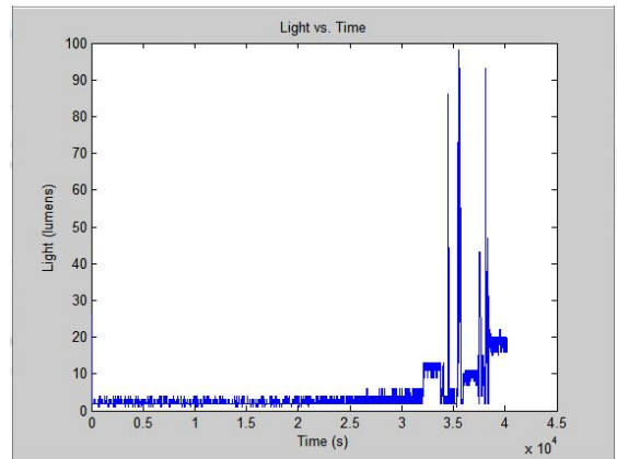
Figure 23: Data captured from live test of light
