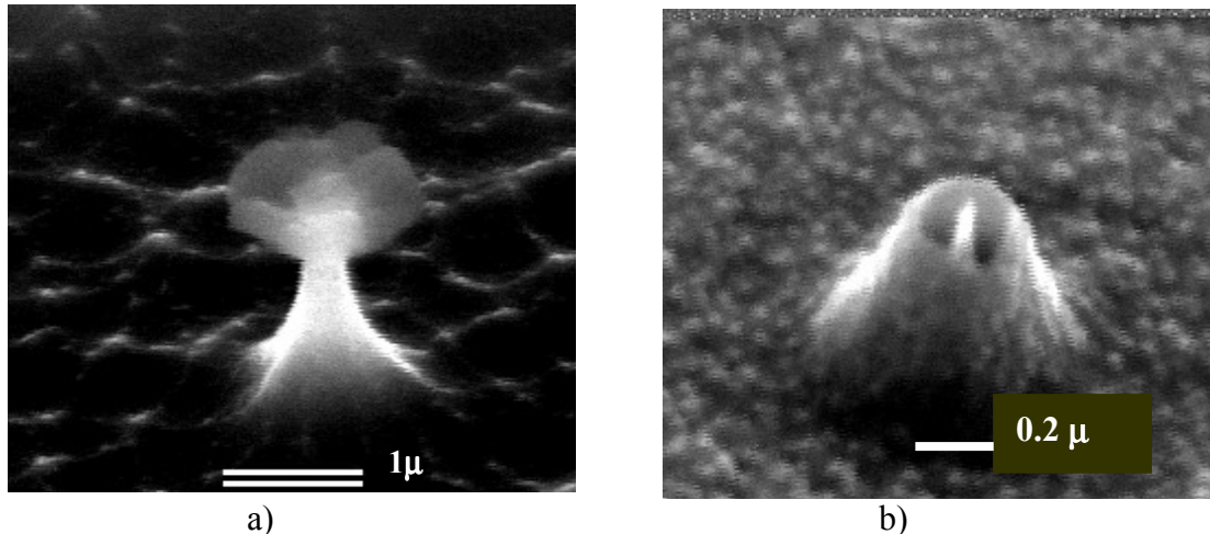
Figure 1. a) Polycrystalline silicon tip before oxidation sharpening. Oxide cap is on top of the tip. b) A completed volcano-type field-emission cell, having 0.3 \mu gate opening and approximately 15 nm tip curvature radii.
