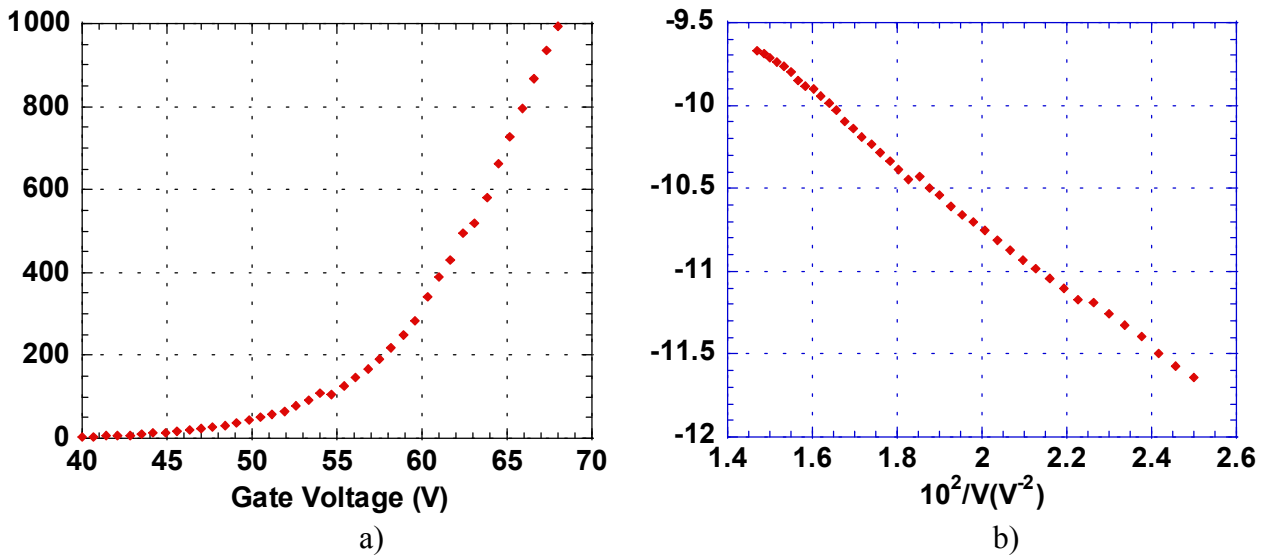
Figure 2. a) Anode current vs. gate voltage plot and b) the Fowler-Nordheim plot for the anode current up to 1000 nA.
